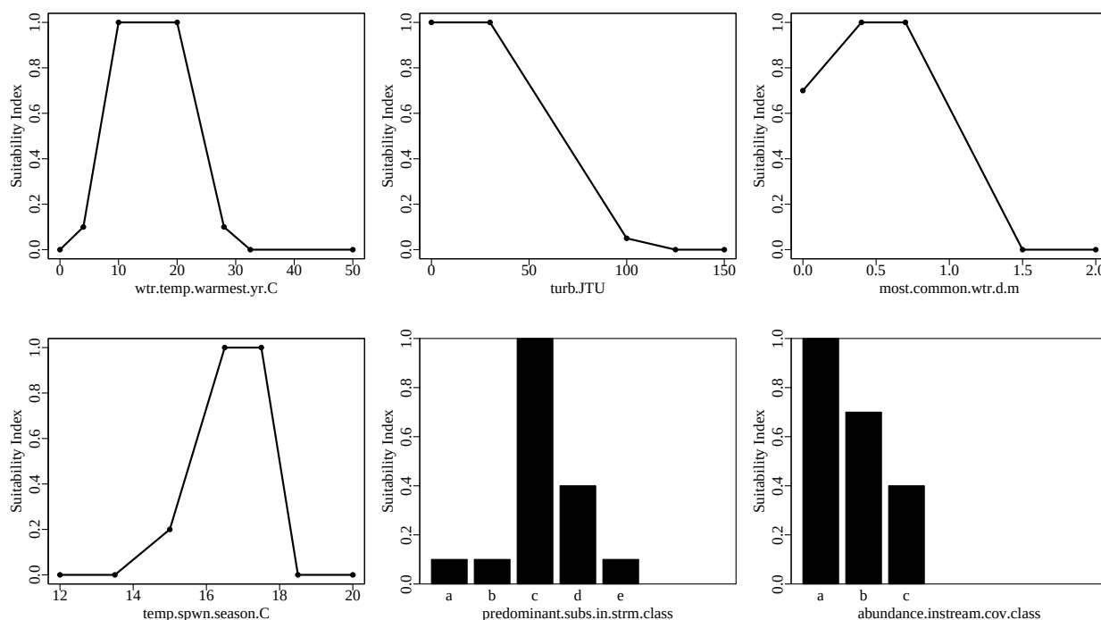
Figure 1. Suitability index graphs for variables included in the fallfishRivNoSpwn model in ecorest .
