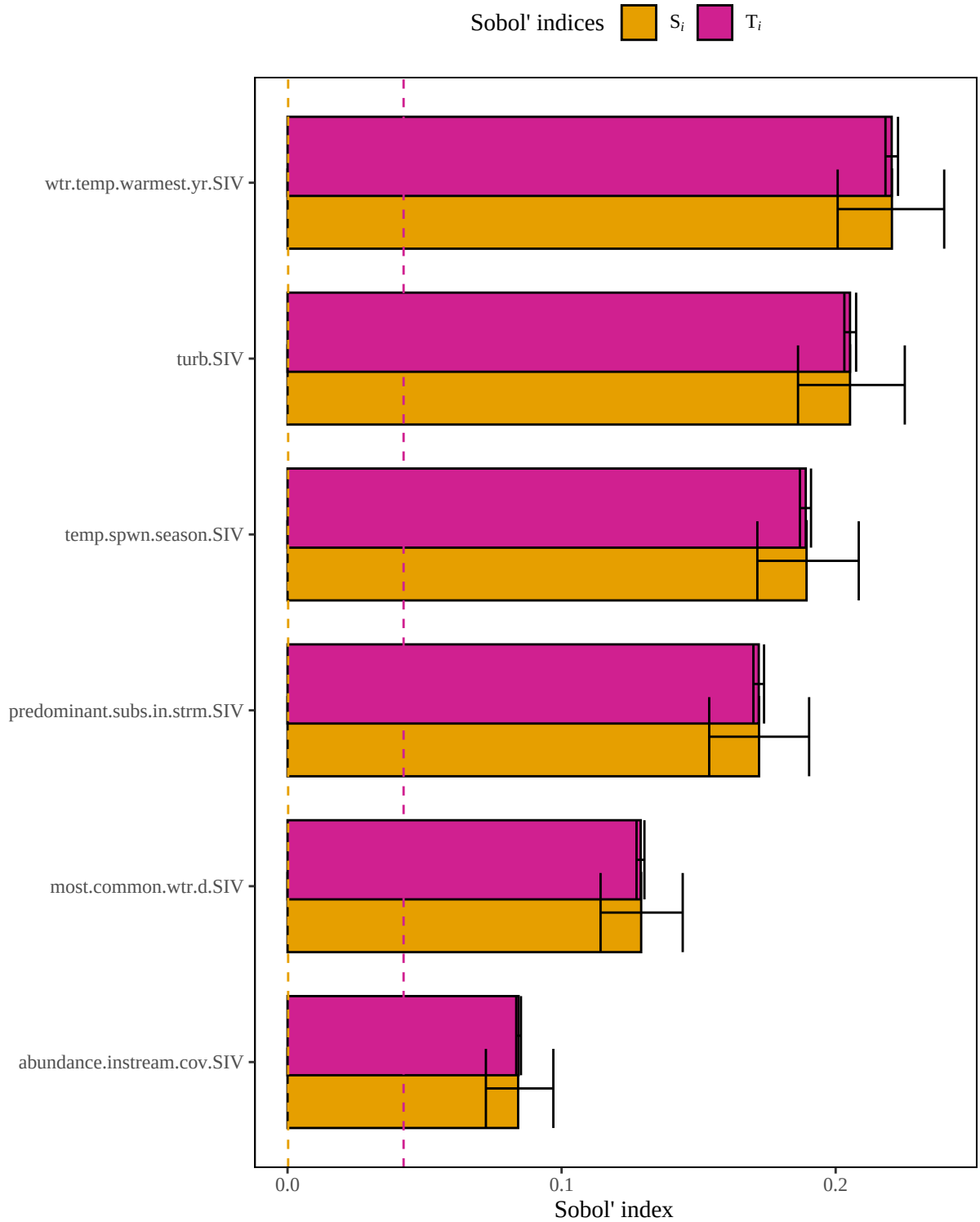
Figure 4. Results of a sensitivity analysis for the fallfishRivNoSpwn model based on an arithmetic mean structure. Dashed lines represent baseline numerical approximation error for S_i and T_i ( i.e. , dummy variables).
